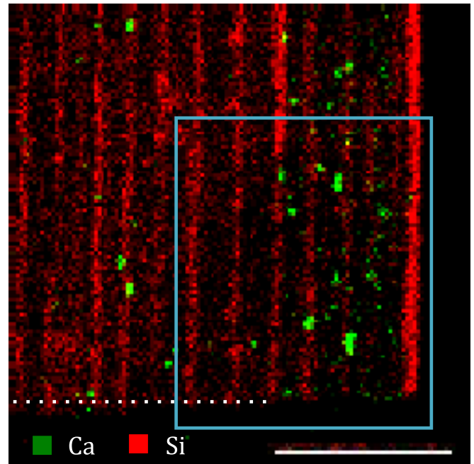
Fig. 3 Micro X-ray fluorescence spectroscopy (micro-XRF) (1 px = 20 \mu\text{m} , field of view (FOV) = 2.56 \times 2.56 \text{mm}^2 ) 2D imaging of a dried leaf treated with silicon 1.5 mM (bar, 1000 \mu\text{m} ) showing the distribution of silicon (Si) (red) and calcium (Ca) (green); the square is the position of the micro-computed tomography (micro-CT) image shown in Fig. 4(b).
