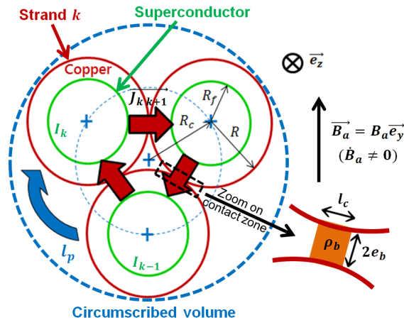
Fig. 1. Scheme showing the cross-section geometry of a triplet ( N=3 )
