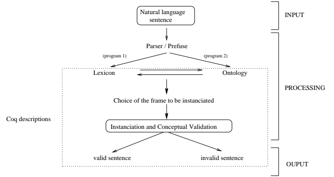
Fig. 2. Overview of the application based on a Coq analysis
