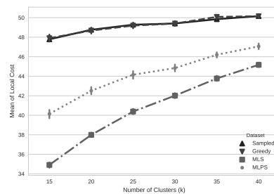
(b) Locality costs using RANDOM clusterings. The greedy and sampled curves almost perfectly fit each other.
