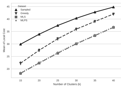
(a) Locality costs using K-MEDOIDS clusterings. The MLS and MLPS curves almost perfectly fit each other.
