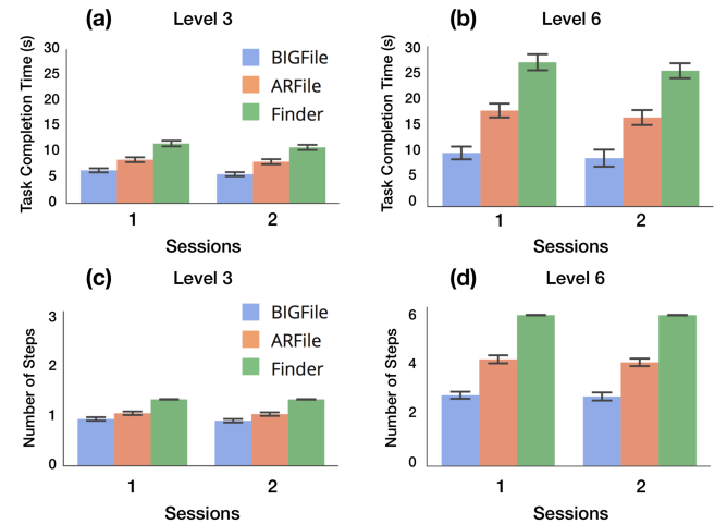
Figure 6. Task Completion Time (a, b) and number of steps (c, d) for the 3 interfaces, in 2 sessions, at levels 3 & 6, with 95% confidence intervals.
