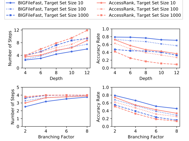
Figure 4. Simulations of BIGFileFast vs. AccessRank for a Zipf distribution ( s = 1 ) and three target set sizes (10, 100, 1000). The plots show the number of steps (left, lower is better) and accuracy rates (right, higher is better) as a function of depth (top) and branching factor (bottom).
