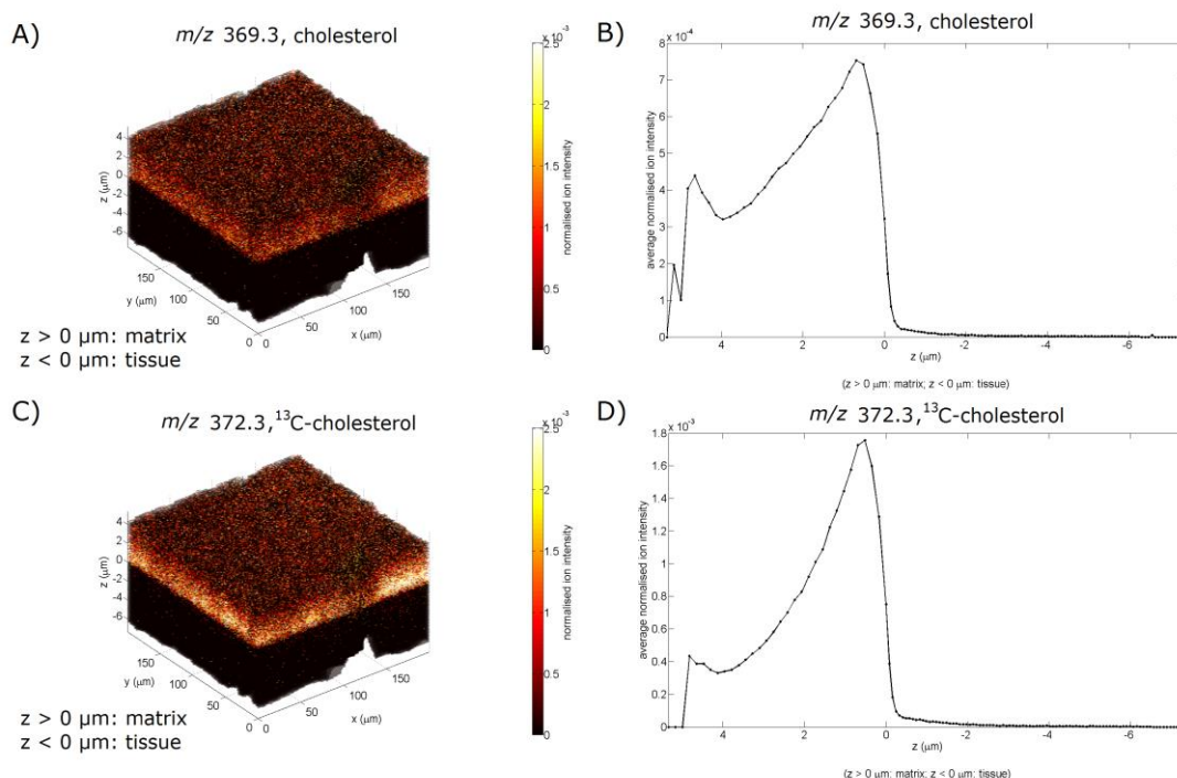
FIGURE 4. 3D ToF-SIMS image data showing the distribution of cholesterol and ^{13}\text{C} -cholesterol in a liver tissue sample coated with DHB. A) 3D Ion image for m/z 369.3, the [\text{M}+\text{H}-\text{H}_2\text{O}]^+ fragment of cholesterol. B) Depth profile of the m/z 369.3 ion. C) 3D Ion image for m/z 372.3, the [\text{M}+\text{H}-\text{H}_2\text{O}]^+ fragment of cholesterol-2,3,4- ^{13}\text{C}_3 . D) Depth profile of the m/z 372.3 ion.
