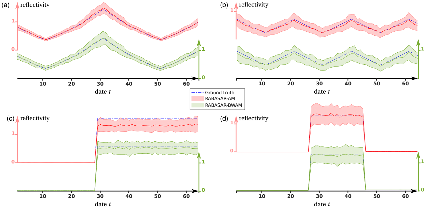
Fig. 6: Evaluation of RABASAR estimators in 4 different change scenarios: typical temporal variations of reflectivities in (a) farmland areas; (b) forest areas; (c) urban areas when a new building appears; (d) urban areas with an appearing then disappearing structure. The mean and 1\sigma confidence interval are displayed for RABASAR-AM (top curve) and RABASAR-BWAM (bottom curve).
