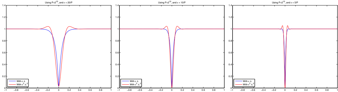
Figure 3: Comparison of optimal profiles u_{\gamma_1}^\varepsilon in dimension 1, for different values of \varepsilon and using the two different models. From left to right: \varepsilon = 20/P , \varepsilon = 10/P , \varepsilon = 5/P with P = 2^{10} .
