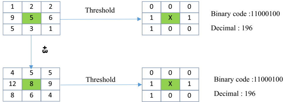
Fig. 3 Diagram of the LBP descriptor and gray-scale invariant
