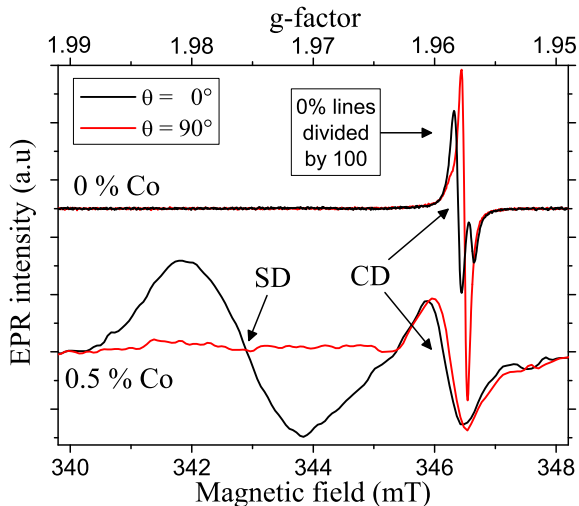
Figure 4: (colour online) Anisotropy of the EPR CD signal in pure (0% Co) and Co-doped (0.5%) samples, with respect to the magnetic field orientation, recorded at T = 6 K. Sapphire defect (SD) signal present in the 0.5% sample is shown for the \theta = 0^\circ orientation.
