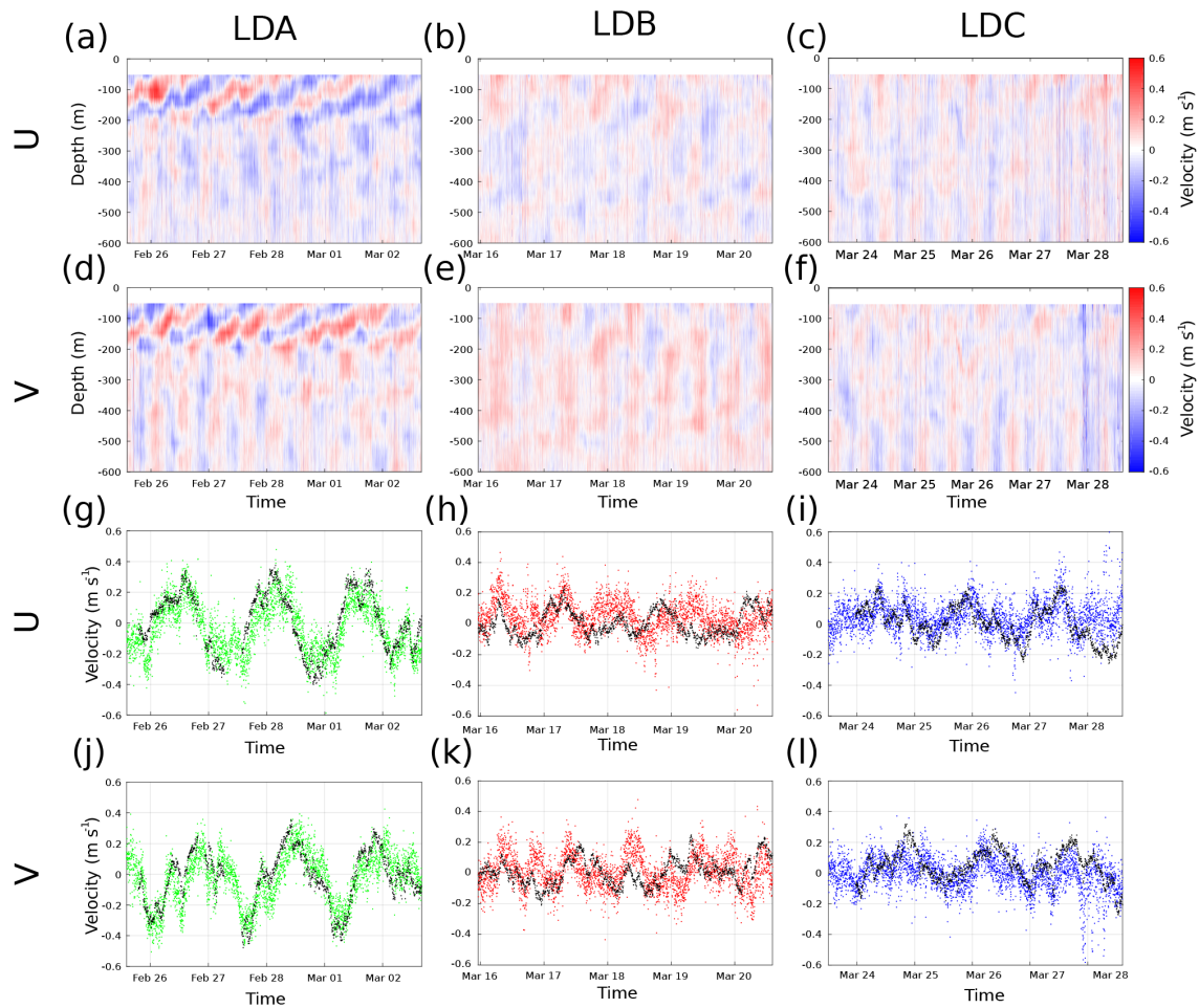
Figure 14. Time series of 38 kHz SADCPC u and v components over depth for (a, d) LDA, (b, e) LDB, and (c, f) LDC. Comparison of 55 m Aquadopp u and v components with 52 m SADCPC u and v for (g, j) LDA, (h, k) LDB, and (i, l) LDC. Aquadopp measurements shown in black, SADCPC measurements follow the color code. Units are in \text{m s}^{-1} .
