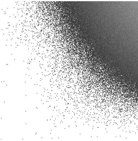
Figure 1: A simulation of a random point measure \bigsqcup_{n \geq 0} \mathbf{Z}_n on \mathbb{R}_+ \times \mathbb{R}_+ with self-similarity exponent -1 .
