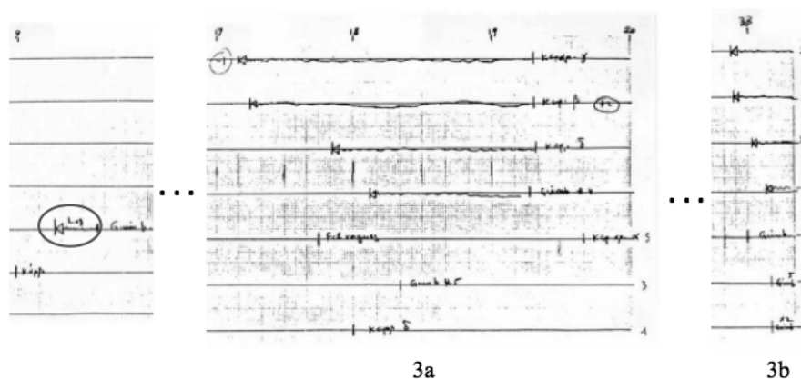
Figure 9. Peaks 3a and 3b in La Légende d'Eer compositional score.
