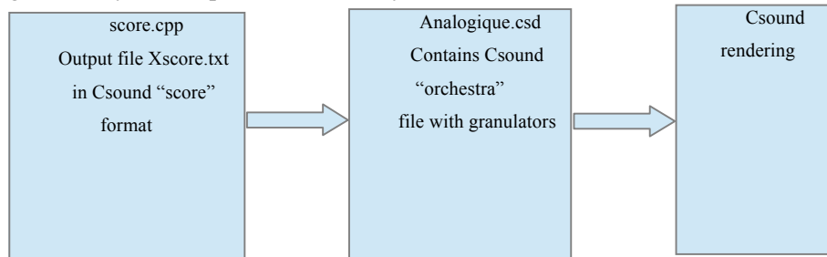
Figure 7. Two step process: score generator and granular synthesis
