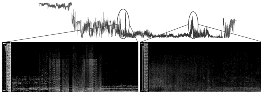
Figure 8. Peaks 3a (16'23'' – 20'30'') and 3b (16'23'' – 20'30'') in La Légende d'Eer . [The original is in colour]
