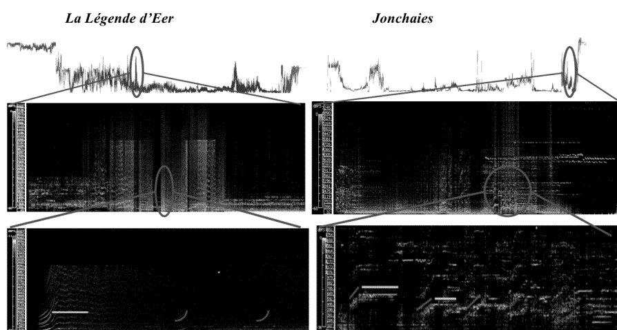
Figure 16. Upper graphics: Piece's Global Maps - La Légende d'Eer (left), Jonchaies (right). Middle Graphics: Peaks 3a (16'23'' – 20'30'') in La Légende d'Eer and 3c in Jonchaies (12'19'' – 15'58''). Bottom graphics: Zoom in the Peaks' Internal structure: Peaks 3a (18'44'' – 18'51'') in La Légende d'Eer and 3c in Jonchaies (14'18'' – 14'40''). [The original is in color]
