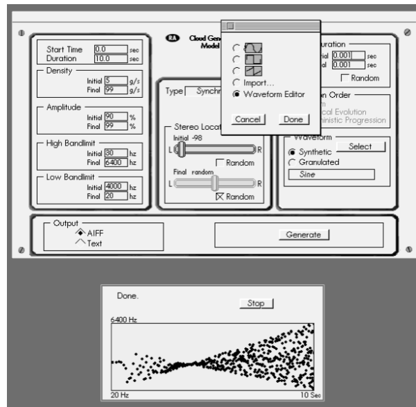
Figure 2. The Cloud Generator app in action 1995.
