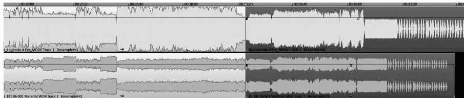
Figure 4. Comparison of channel 1 of the 2003 digitized Paris tape (upper channel) used for the Mode record CD with the Cologne material tape 1 (lower channel).
