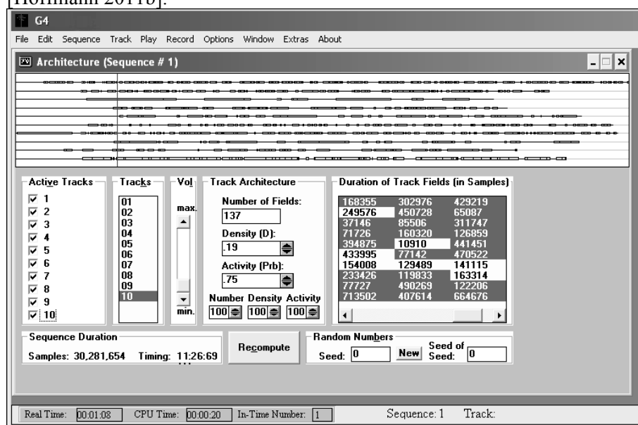
Figure 2. Example of a composition made with the New GENDYN Program: G4 by Paul Doornbusch (1999). One can see the duration structure („score synthesis“) of the entire piece with its „patches“ of sound distributed over 10 simultaneous „voices“. Note that pitch is not part of score synthesis but an emergent by-product of sound synthesis, which is not shown in this picture. The picture is taken from Paul's PhD thesis [Doornbusch 2010]
