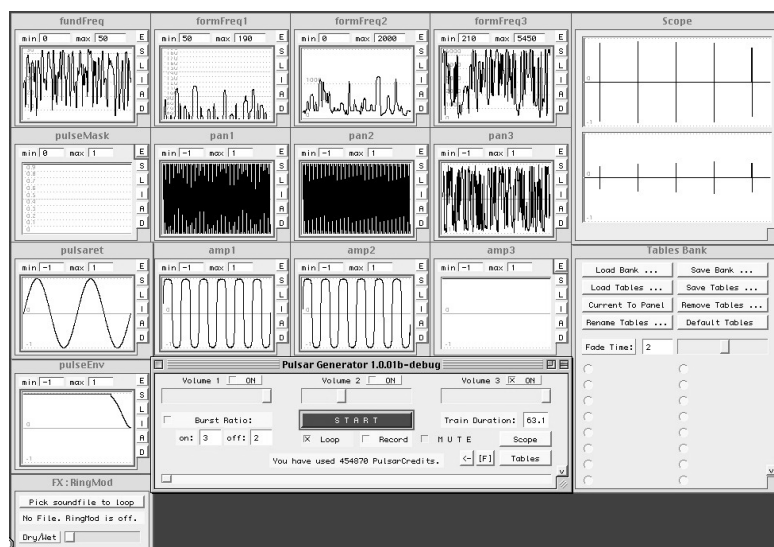
Figure 7. The PulsarGenerator screen focused on envelope control of particle synthesis. (The original is in colour)
