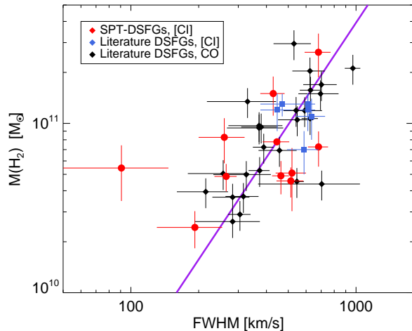
Figure 7. The observed linewidth (full width half maximum, FWHM), plotted against total H_2 mass for SPT-DSFGs and literature DSFGs. For SPT-DSFGs (red), and DSFGs taken from Alaghband-Zadeh et al. (2013) (blue), linewidths and H_2 masses are derived using [C \text{I} ]. For the literature DSFGs, taken from Bothwell et al. (2013), linewidths and H_2 masses are derived using either CO(2 – 1) or CO(3 – 2). The purple line represents a simple dynamical mass model (given in Eq. 8).
