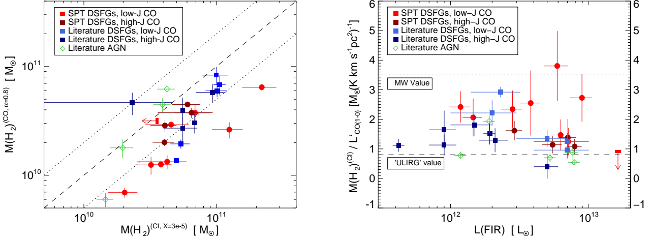
Figure 6. Left Panel: Comparison of molecular hydrogen masses, derived via [CI] and CO emission, for the SPT DSGFs in this paper and the DSGFs in Alaghband-Zadeh et al. (2013) with both [CI] and CO observations. To derive CO-based \text{H}_2 masses, we have assumed \alpha_{\text{CO}} = 0.8 . The dashed diagonal line indicates equal masses, while the dotted lines show a factor of two variation each way. DSGFs for which a higher- J CO line has been used to infer a gas mass have been plotted using darker colours. Right Panel: Ratio between [CI]-derived molecular gas mass and \text{CO}(1-0) luminosity, for the same galaxies. This ratio can be interpreted as giving the CO-to- \text{H}_2 conversion factor \alpha_{\text{CO}} . All (but one) SMGs in both samples have implied values of \alpha_{\text{CO}} far above the canonical ‘ULIRG’ value, and several SPT-DSFGs have an \alpha_{\text{CO}} comparable to that of the Milky Way.
