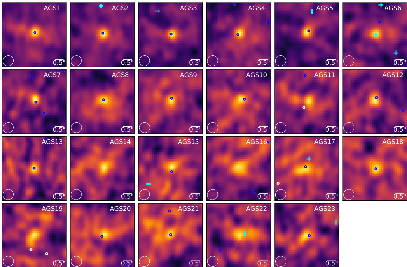
Fig. 7. ALMA 1.1 mm continuum maps for the 23 detections tapered at 0.60 arcsec. Each 3'' \times 3'' image is centred on the position of the ALMA detection. Cyan double crosses show sources from the GOODS- S CANDELS catalogue. White circles show sources from the ZFOURGE catalogue. Blue circles show common sources from both optical catalogues (i.e. sources with an angular separation lower than 0''.4 ). The shape of the synthesized beam is given in the bottom left corner.
