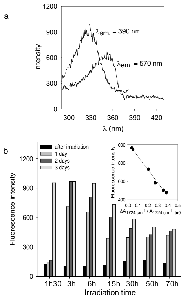
Fig. 10. (a) Excitation spectra of an irradiated PETTA/2EEEE film containing 1 wt% of ZnO QDs after storage in the dark at room temperature during 3 days. (b) For each irradiation time in SEPAP 14/24 ( \lambda \geq 300 nm and 40 °C), evolution of the fluorescence intensity at 570 nm ( \lambda_{\text{exc.}} = 350 nm) of a composite film after irradiation and followed with a storage during 1, 2 and 3 days in the dark. Inset: Correlation between the maximum fluorescence intensity value and the decrease of the ester groups (band at 1724 \text{cm}^{-1} ).
