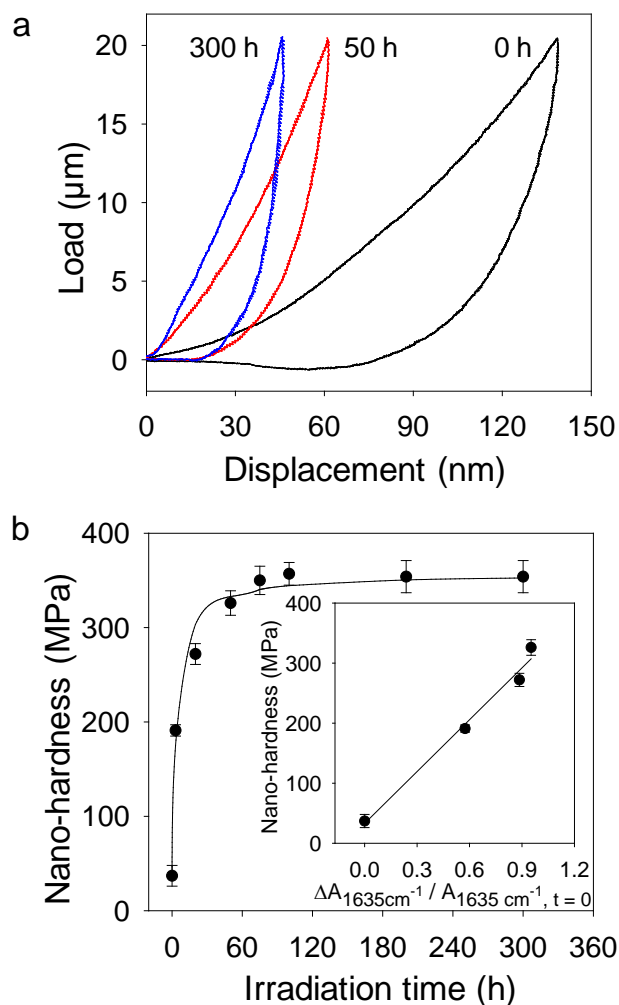
Fig. 5. (a) Force-displacement curves of PETTA/2EEEEA polymer at 0, 50 and 300 hours of irradiation in SEPAP 14/24 ( \lambda \geq 300 nm, 40 °C). (b) Kinetic evolution of calculated nano-hardness for a constant load of 20 \mu\text{N} upon irradiation of PETTA/2EEEEA polymer. Inset: Correlation between the nano-hardness and the decay of the residual vinyl groups (band at 1635\text{ cm}^{-1} ).
