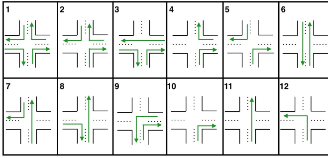
Fig. 3. Possible patterns in the modeled crossroad
