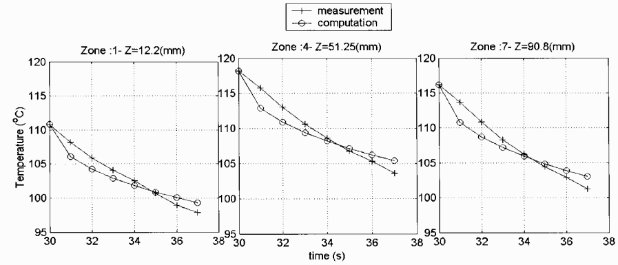
Figure 6. Comparison between measured and computed preform temperatures
