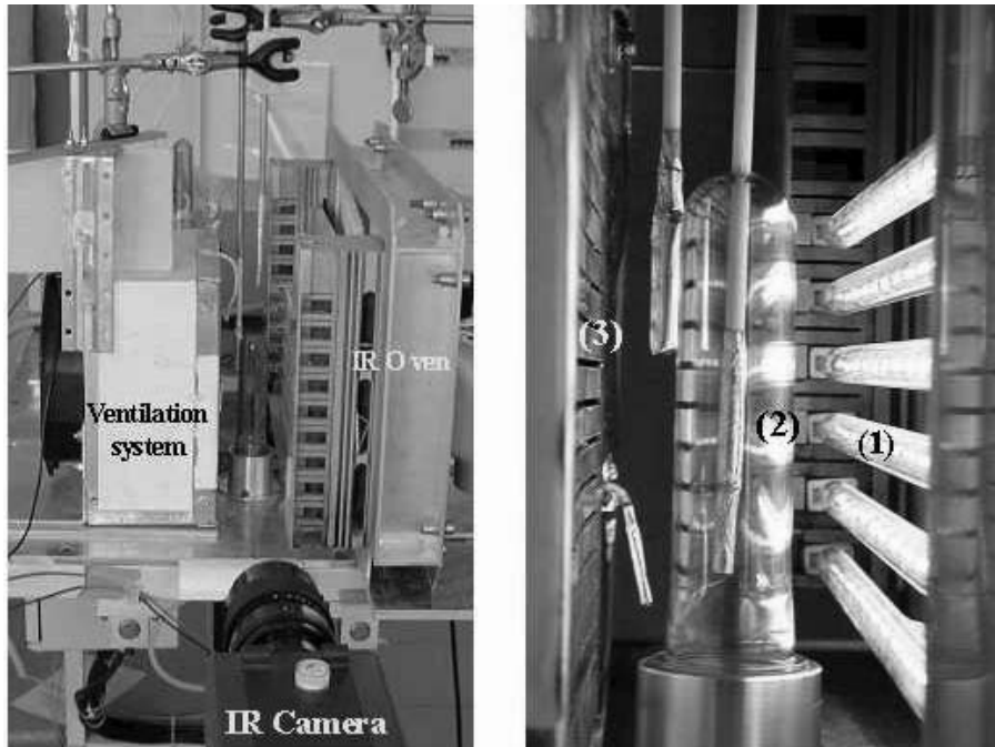
a) General view of the oven
