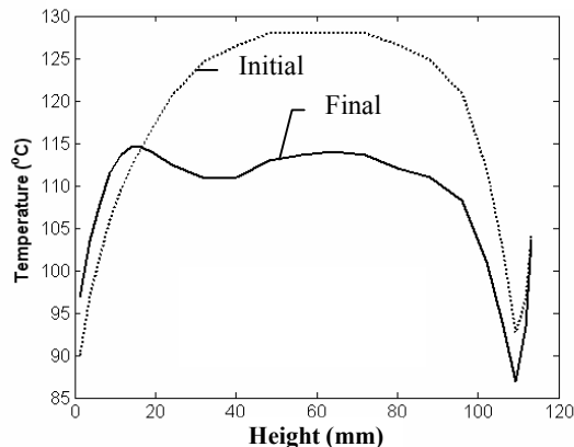
Fig. 6. Front surface temperature distribution after 15 s heating, computed with Termoray. Initial and updated oven geometry.
