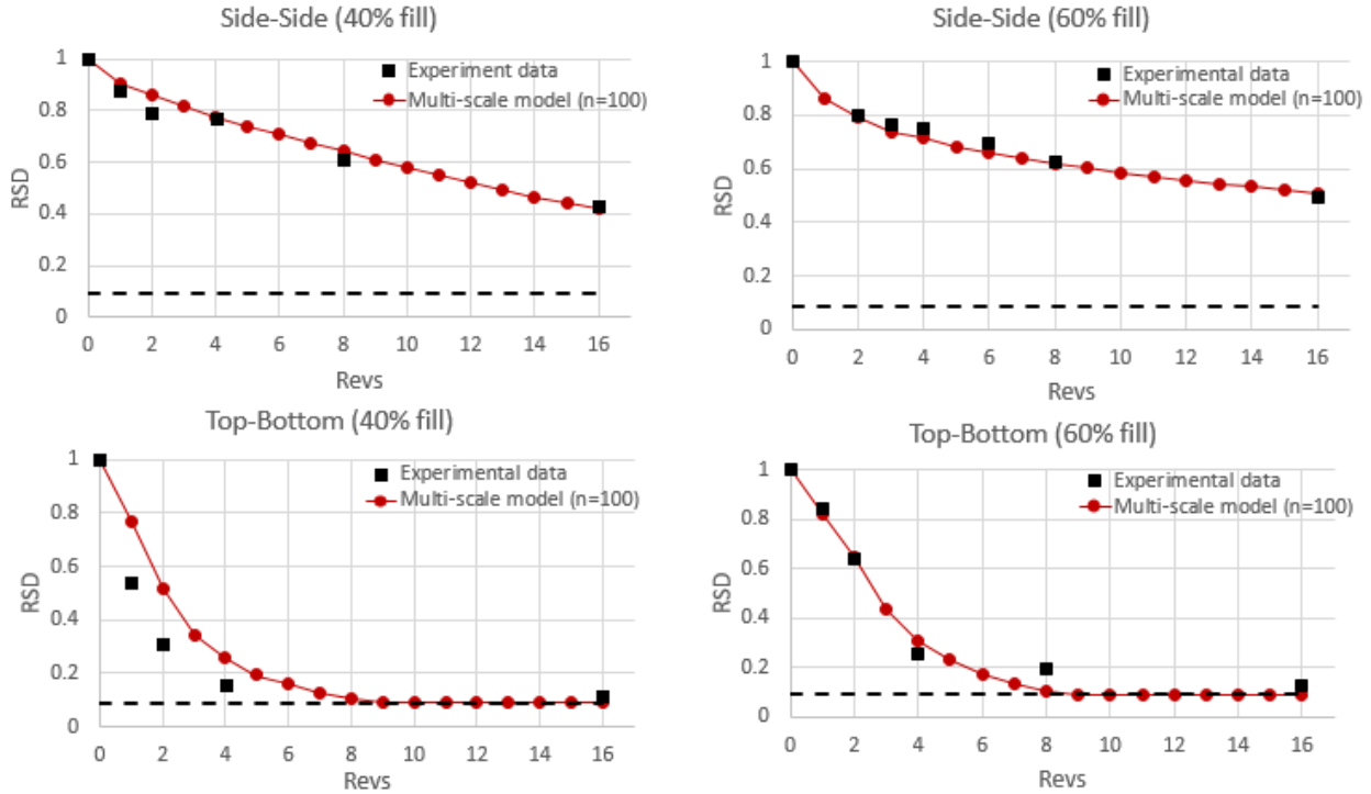
Figure 12. Mixing state comparison between published experimental results and the multi-scale model predictions. The random mixing state is represented by horizontal dashed lines and the spanwise diffusion constant is k_1 = 0.01 .
