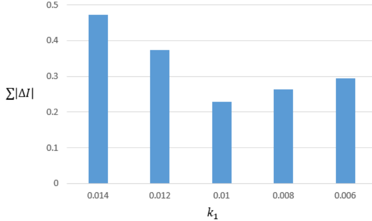
Figure 8. Sum of the absolute differences between the segregation intensities measured from experiments and computed from the 2-D multi-scale model for different k_1 values.
