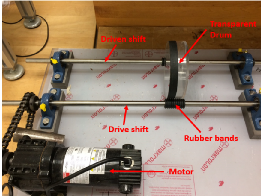
Figure 5. The rotating drum experiment setup.
