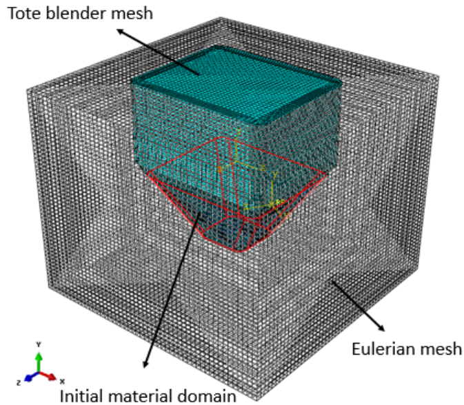
Figure 2. A schematic of the FEM model domain. The Eulerian mesh is shown in grey, the Tote blender mesh is shown in blue, and the outlines of the initial material domain are shown in red.
