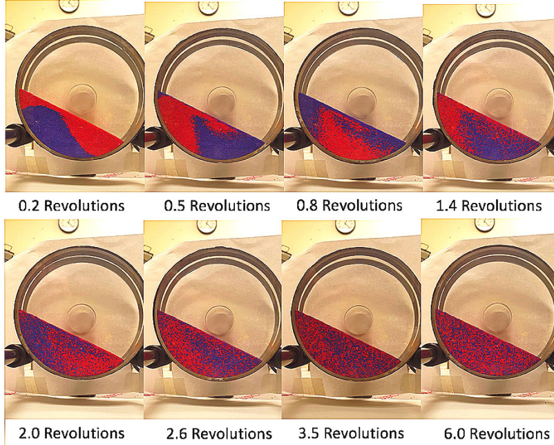
Figure 6. Snapshots showing the state of particle mixing for different numbers of drum revolutions in the rotating drum experiments.
