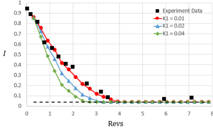
Figure 7. Segregation intensity with respect to the number of drum revolution for the experiment and the 2-D multi-scale model using different k_1 values.
