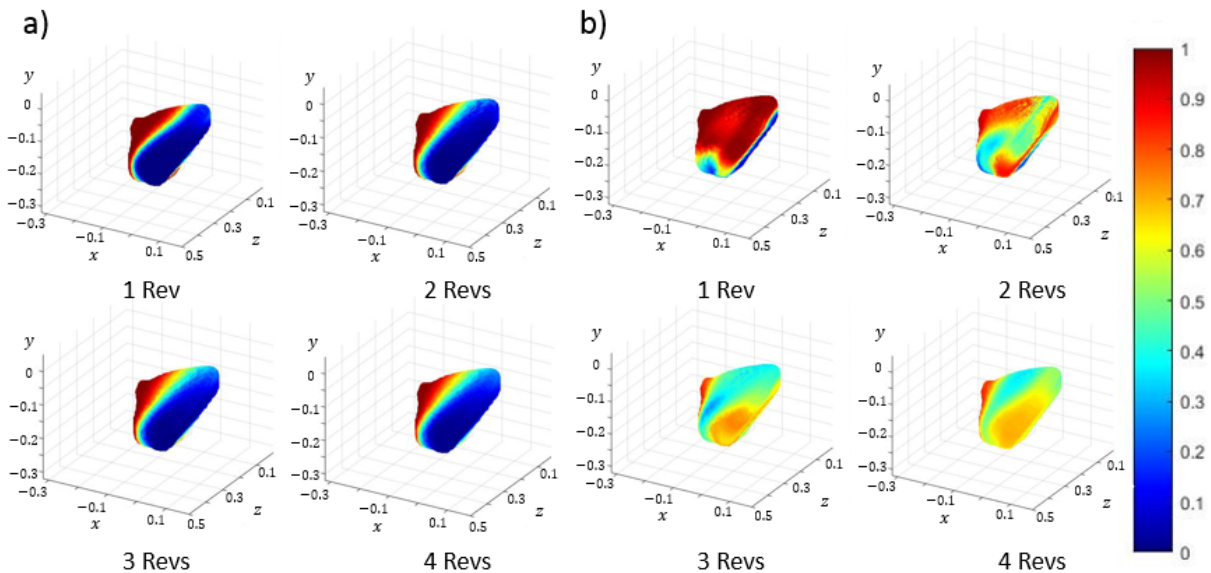
Figure 11. Snapshots showing the state of mixing at the end of each revolution for (a) left-right loading and (b) top-bottom loading and 40% fill. The vertical color scale is the red particle concentration for (a) and (b).
