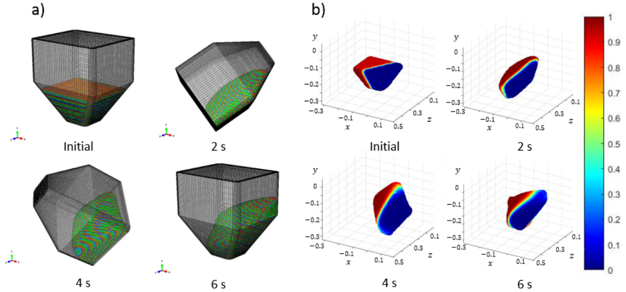
Figure 10. Snapshots showing the change of the material domain in the FEM simulation (a) and multi-scale model (b) for left-right loading and 40% fill. The vertical color scale in (b) is the red particle concentration.
