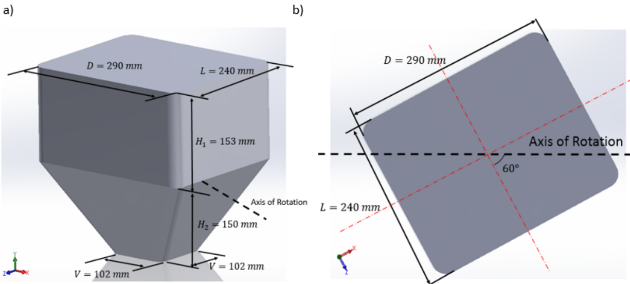
Figure 1. Dimensions of the GEA Gally Tote blender used in the FEM simulation.
