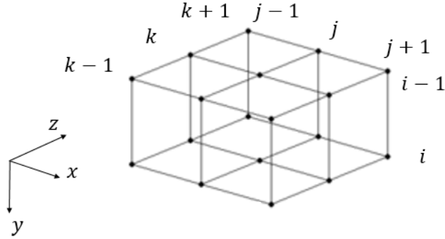
Figure 4. Computational molecule for the second-order, three-dimensional Taylor Lax-Wendroff scheme.
