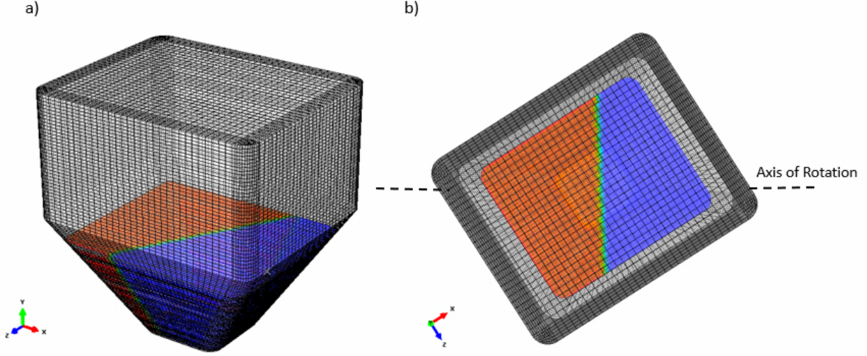
Figure 3. Initial material concentration for a simulation with left-right loading. The color represents field variable value from zero (blue) to one (red). The materials in this simulation have homogeneous properties, except for color.
