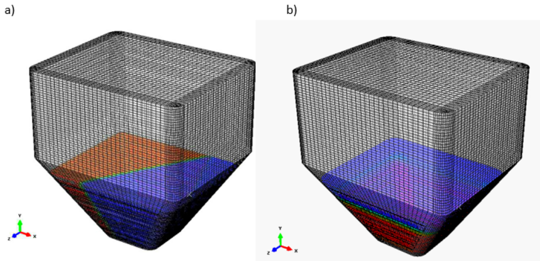
Figure 9. The left-right (a) and top-bottom (b) initial loadings for 40% fill.
