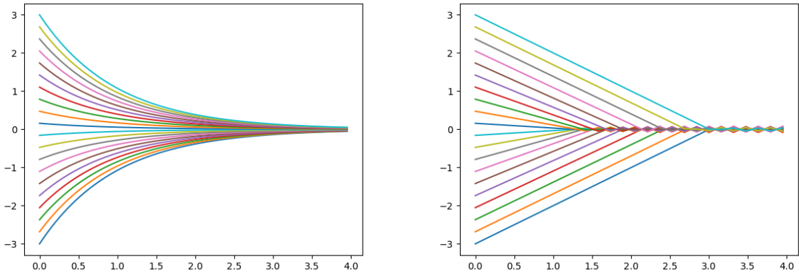
Figure 1: Trajectories of particles for the potential W(x) = x^2
