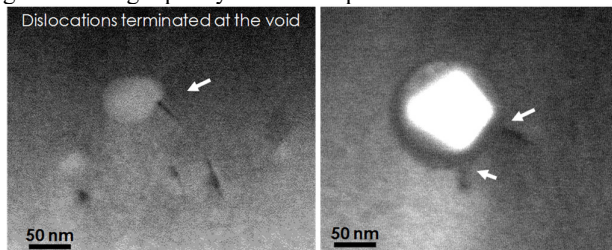
Fig. 5 STEM images shows the termination of a dislocation segment in the nanovoid area.
