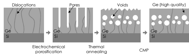
Fig. 1 Schematic illustration of dislocation trapping by nanovoids approach.
