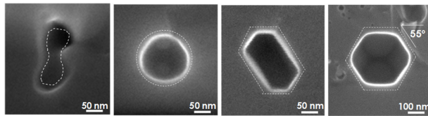
Fig. 3. Different types of the void shapes observed during the annealing of Ge/Si layer (400-700°C) in hydrogen ambient.
