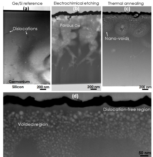
Fig. 4 STEM mixed Dark Field and Bright Field images obtained from irradiated 80 nm Ge/Si sample, (a) reference sample, (b) porous Ge/Si sample, (c) voided Ge/Si sample and (d) higher magnification of (c) indicates the formation of a dislocation-free region at the upper part of the voided region.
