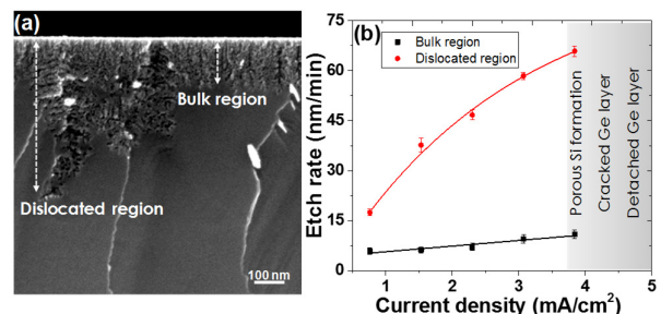
Fig. 2 Cross-section SEM images of porous Ge/Si layer formed at 1.5 \text{ mA/cm}^2 (a) and (b) etch rates versus current density of dislocated and bulk regions in Ge/Si layer.
