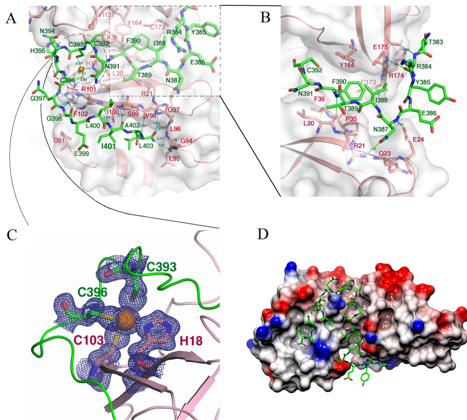
FIGURE 3. the molecular interactions between GRASP55 and Golgin45 C-terminal peptide. A, detailed interactions between GRASP55 and Golgin45 C-terminal residues at the conventional peptide-binding groove of the PDZ1 domain. The residues involved in the PDZ1-Golgin45 peptide interaction are shown with a stick model in which GRASP55 and Golgin45 peptide backbones are colored pink and green , respectively, and nitrogen and oxygen atoms are colored blue and red , respectively. The surface of GRASP55 PDZ1 domain is also illustrated. A zoom of the area in the dashed square is shown in B, whereas a zoom of the area in the dashed circle is shown in C. B, detailed interactions between GRASP55 and Golgin45 C-terminal peptide at the cleft between PDZ1 and PDZ2 domains. The residues involved in the interaction are shown with a stick model. GRASP55 and Golgin45 peptide backbones are colored pink and green , respectively, and nitrogen and oxygen atoms are colored blue and red , respectively. The GRASP55 surface is also illustrated. C, detailed interactions of the zinc finger formed between GRASP55 and Golgin45. Residues involved in the zinc finger are shown with a stick model. Electron density map of the zinc finger and ion are also illustrated (1.5 \sigma ). Zinc ion, GRASP55 and Golgin45 peptide backbones are colored orange , pink , and green , respectively. D, surface topology of the GRASP domain of GRASP55 highlighting the canonical PDZ-peptide binding pocket of PDZ1 and the cleft between PDZ1 and PDZ2. The C-terminal sequence of the Golgin45 peptide is shown with a stick model and colored green . Electrostatic surface potential is shown too.
