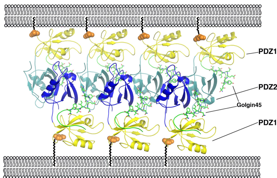
FIGURE 6. Molecular models of GRASP55-Golgin45-mediated mid-cisternae membrane stacking. PDZ1 domains are colored yellow, whereas PDZ2 domains of GRASP55 are colored blue. Golgin45 C-terminal peptides are shown with a stick model and colored green. The ball and zigzag lines represent GRASP55 N-terminal myristoylation. A series of GRASP55 and Golgin45 molecules form ordered membrane-associated protein arrays between two apposing membranes.
