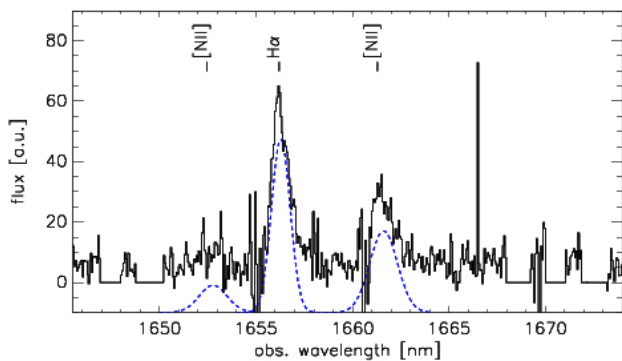
Fig. 2. VLT/X-Shooter spectrum of H\alpha and [N\text{II}]\lambda\lambda 6548,6583 in the lens at z = 1.525 \pm 0.001 . Blue lines show Gaussian line fits. Bright night-sky line residuals are clipped.
