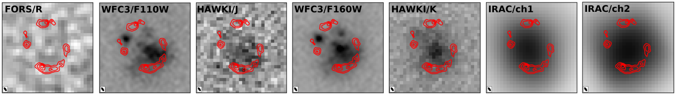
Fig. 1. Left to right: Three arcsecond wide postage stamps of the Ruby in the R , F110W, J , F160W, K , 3.6- \mu\text{m} , and 4.5- \mu\text{m} bands. Contours show the CO morphology from C17 taken with 0.14'' \times 0.06'' beam size (lower left corner of each panel); they start at 3\sigma , and increase in steps of 3\sigma .
