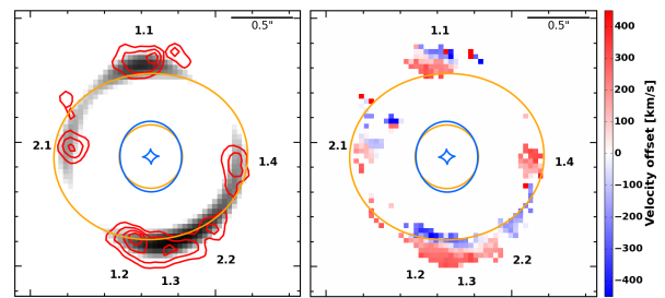
Fig. 3. Left: Reconstructed (grayscale) and observed (contours) \text{CO}(4\rightarrow 3) surface brightness observed with ALMA. Right: \text{CO}(4\rightarrow 3) velocity map of the Ruby. We label the two sets of multiple images; we show the tangential and radial critical curves at z = 1.525 and caustic lines at z = 3.005 as orange and blue lines, respectively.
