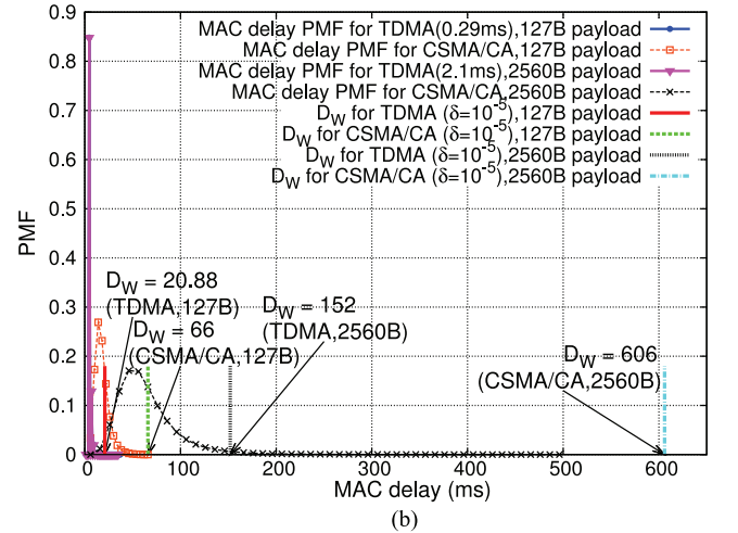
Fig. 8. Worst-case delay bound comparison for different payload sizes for 2-flow 2-relay and 1-flow 3-relay TDMA and CSMA/CA networks. \delta = 10^{-5} . (a) 2-flow 2-relay; and (b) 1-flow 3-relay ( S_{\text{min}} solution).
