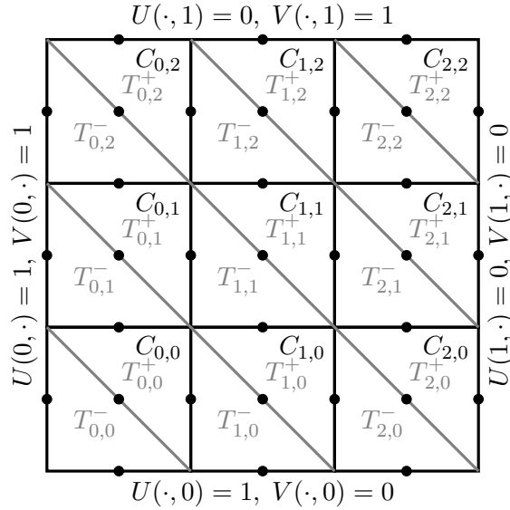
Figure 5: Discretization of the unit square \Omega^h = [0,1]^2 , h = 1/3 using squares C_{0,0}, \dots, C_{2,2} each of size h^2 . Each square C_{i,j} is then divided into an upper triangle T_{i,j}^+ and a lower triangle T_{i,j}^- . The nodes of the mesh, represented as black dots, are in the middle of the edges of the triangles. Note the boundary conditions imposed by the functions U(x,y) and V(x,y) .
