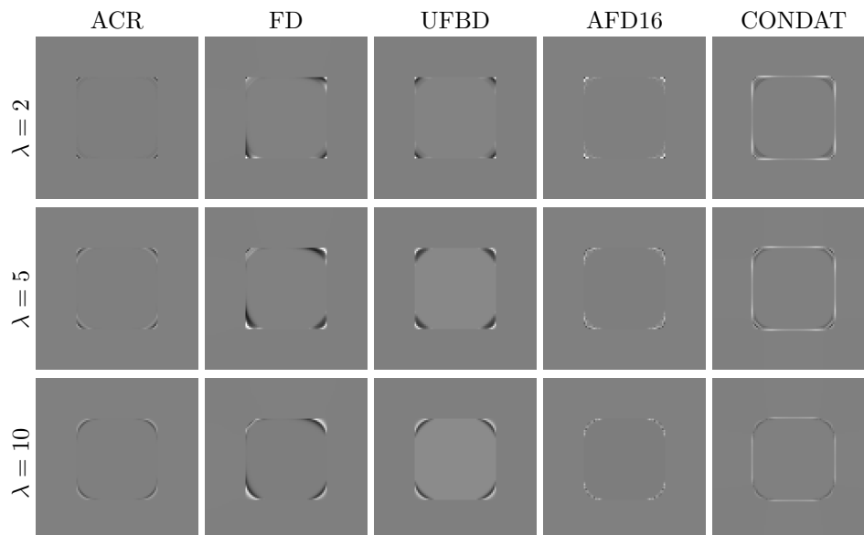
FIG. 11. Error plots of the numerical solutions with respect to the analytical solution. For better comparison, the images are truncated to the range [-0.1, 0.1] and gray corresponds to zero. Note the anisotropic behavior of FD and the significantly larger global error of UFBD.
