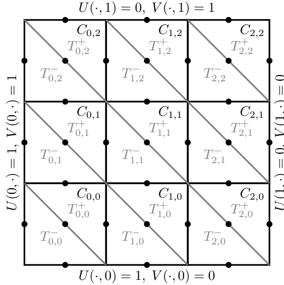
FIG. 5. Discretization of the unit square \Omega^h = [0, 1]^2 , h = 1/3 using squares C_{0,0}, \dots, C_{2,2} each of size h^2 . Each square C_{i,j} is then divided into an upper triangle T_{i,j}^+ and a lower triangle T_{i,j}^- . The nodes of the mesh, represented as black dots, are in the middle of the edges of the triangles. Note the boundary conditions imposed by the functions U(x, y) and V(x, y) .
