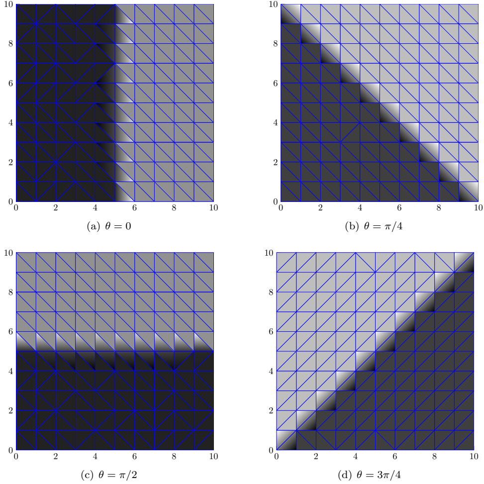
FIG. 7. Recovery of a discontinuity with normal \nu = (\cos \theta, \sin \theta) on a square grid of 10 \times 10 pixels. We plot the image function which is piecewise affine on the triangles together with the triangulation shown in blue. Observe that the triangles are well aligned with the direction of discontinuity while in homogeneous regions the orientation of the triangles is ambiguous.
