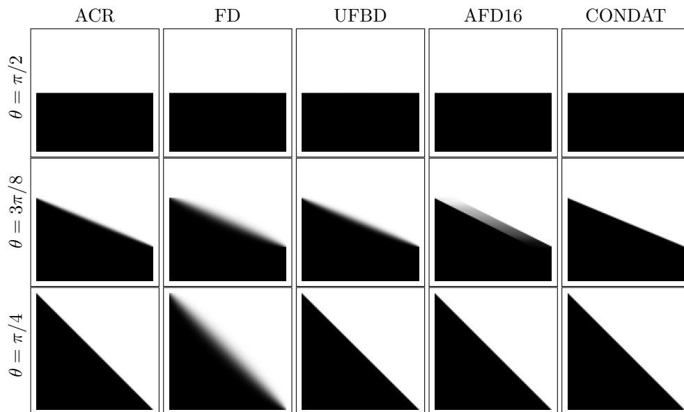
FIG. 8. Images corresponding to the experiments of Table 1. Note the significantly more blurry results of FD and the “failure” of AFD16 to recover a straight line with angle \theta = 3\pi/8 .
