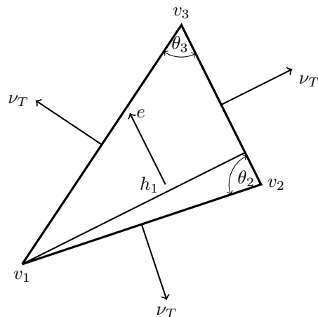
FIG. 3. A triangle T = (v_1, v_2, v_3) \in \mathcal{T}^h together with its outer normals \nu_T , the normalized edge direction e = (v_3 - v_2)/|v_3 - v_2| shown and the two angles \theta_3 = \widehat{v_1 v_3 v_2} and \theta_2 = \widehat{v_3 v_2 v_1} .
