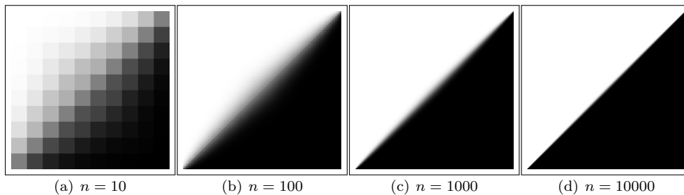
FIG. 6. The smooth transition for different numbers of n , where we only plot the values v_{i+1/2, j+1/2} . Observe that only for a very fine mesh ( n = 10000 ) we obtain a reasonably sharp transition.
