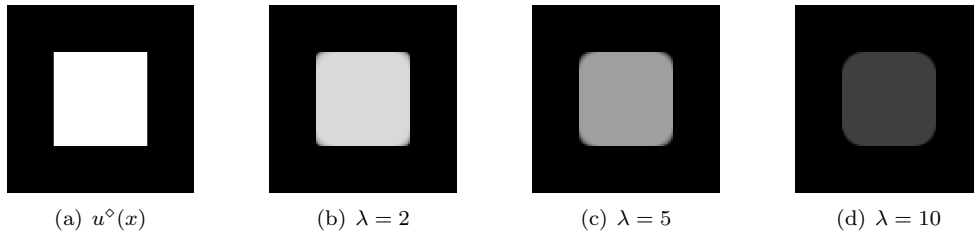
FIG. 10. Original square u^\diamond(x) , and ground truth solutions u(x) for different values of \lambda .
