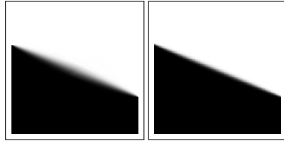
FIG. 13. Left: the variant (B.2), right: the ACR result of Fig. 8.
