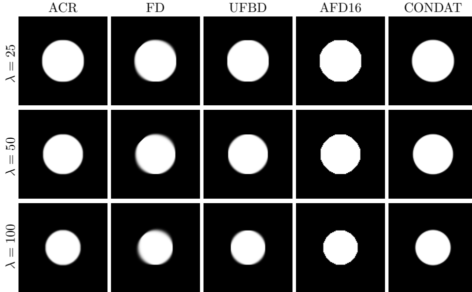
FIG. 9. Image corresponding to the experiments in Table 2. Note the anisotropic behavior of FD and the polygonal behavior of AFD16.
