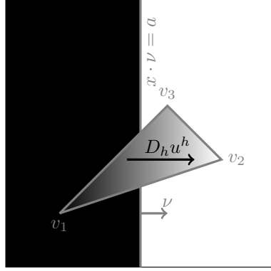
FIG. 4. The figure shows the function u^h and its gradient for one triangle T = (v_1, v_2, v_3) approximating the characteristic function of the half space x \cdot \nu > a with \nu = (1, 0) and a \in \mathbb{R} . The function u^h inside the triangle is affine with a gradient D_h u^h which is simply a multiple of the normal \nu .
