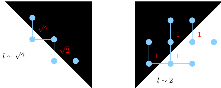
FIG. 1. How J_h would measure a sharp slanted edge: on the left, we get the correct measure, on the right the result is biased by a factor \sqrt{2} , while a smoothed edge in the same direction can have a much lower energy. This explains why discrete minimizers of this approximation will have sharp edges in some orientation, and smoother edges in other.
