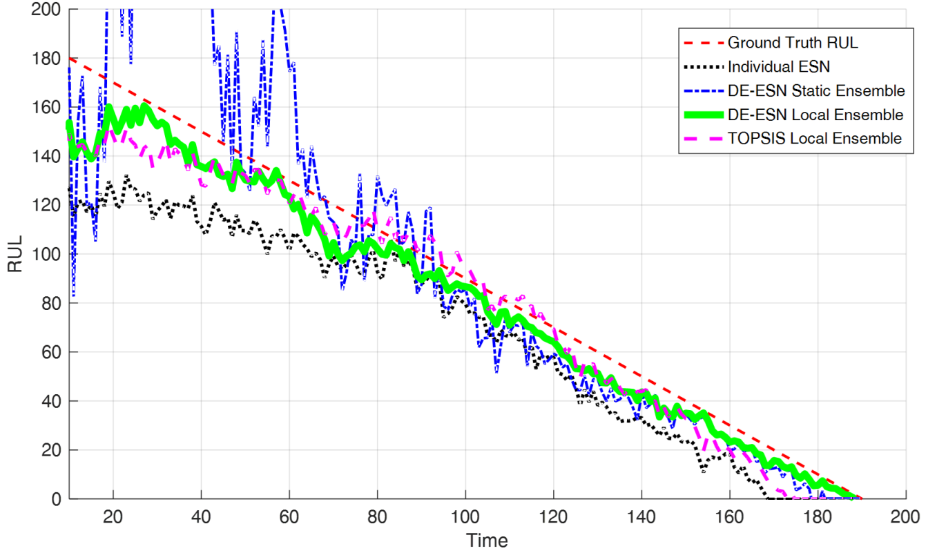
Figure 12. Comparison between the RUL prediction provided by the best ESN individual model (dotted line), the DE-ESN static ensemble (dash-dotted line), the TOPSIS local ensemble (dashed line) and the proposed DE-ESN local ensemble (solid line)
