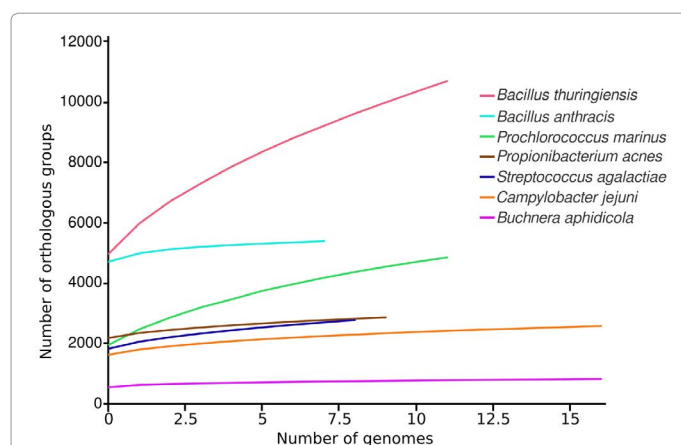
Figure 1: Pan-genome curves of seven different bacterial species. The average pan-genome size (i.e. the average number of total orthologous groups) is shown for the indicated number of genomes.
