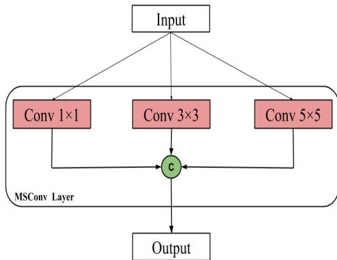
Figure 5: MultiScale Kernel Convolutional Layer
