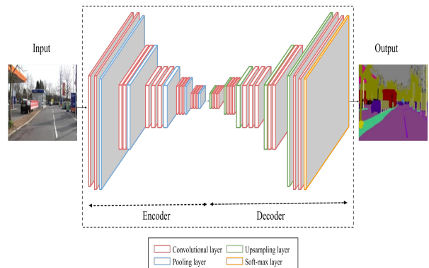
Figure 2: Example of SegNet architecture
