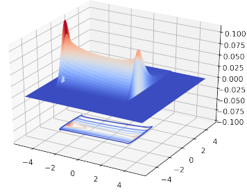
(b) joint distribution of f_{1,2}(\mathbf{y}_n, \mathbf{y}_{n+1}) .
