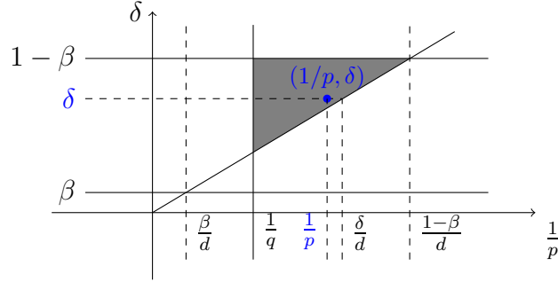
FIGURE 1. The set K(\beta, q) for d > 1 . Given any couple \beta, q that satisfies the assumptions, the grey region shows all possible \delta, p .
