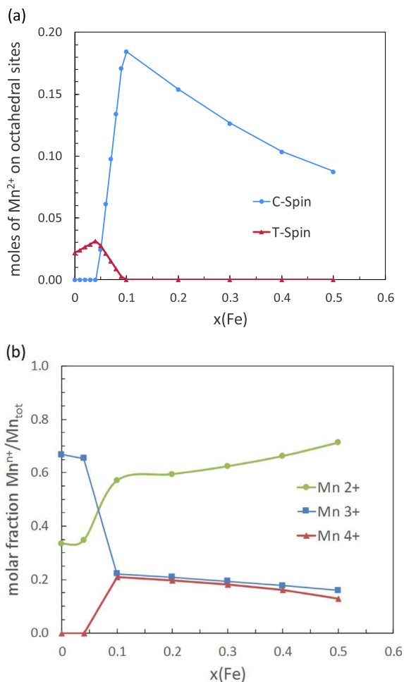
Fig. 13. (a) Evolution of the amount of Mn 2+ on octahedral sites of the spinel phases with Fe content, at 1050 °C. (b) Evolution of the oxidation number of Mn cations in the spinel phases with Fe content, at 1050 °C.
