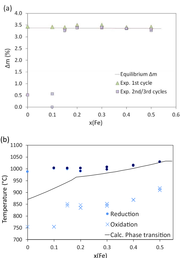
Fig. 12. (a) Evolution of experimental \Delta m (%) during reduction compared to theoretical \Delta m ( p\text{O}_2 = 0.20 atm), (b) Experimental temperatures at peak reaction rate for manganese-based oxides in 20% \text{O}_2/\text{Ar} and comparison with the calculated temperature of the Bixb/Spinel transition.
