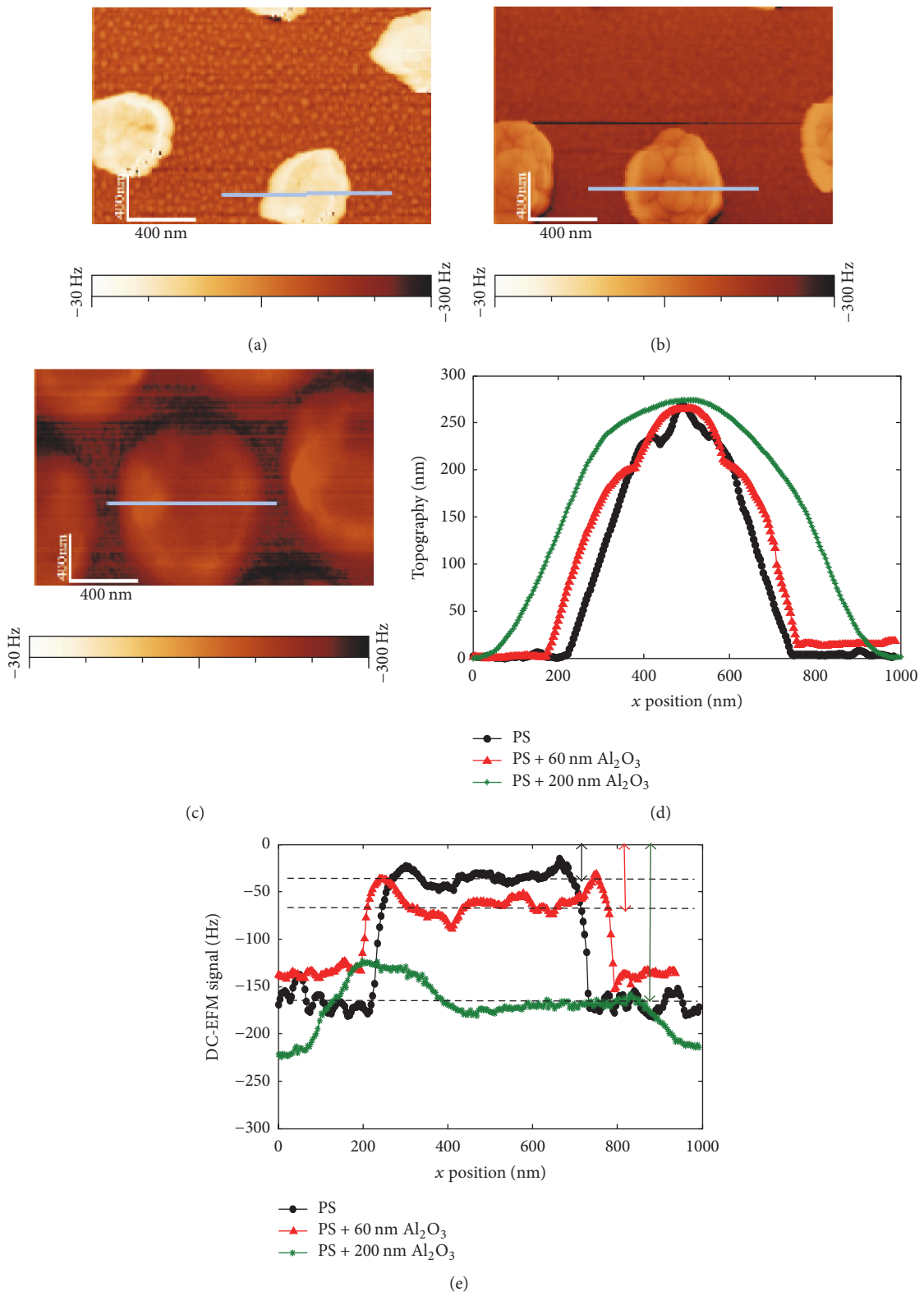
FIGURE 9: (a), (b), and (c) EFM G_{DC} detection electrical signal for PS and PS with 60 nm and 200 nm \text{Al}_2\text{O}_3 , respectively; (d) Cross-sectional topography profiles and (e) EFM signal for studied PS particles at V_{DC} = 5 V and z = 26 nm. Reprinted with permission from [20]. Copyright IEEE 2016.
