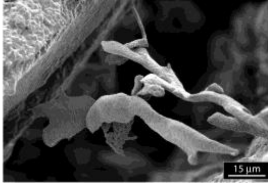
Figure 12: SEM micrograph of ceramic bridges observed for slow freezing of highly concentrated slurries.
