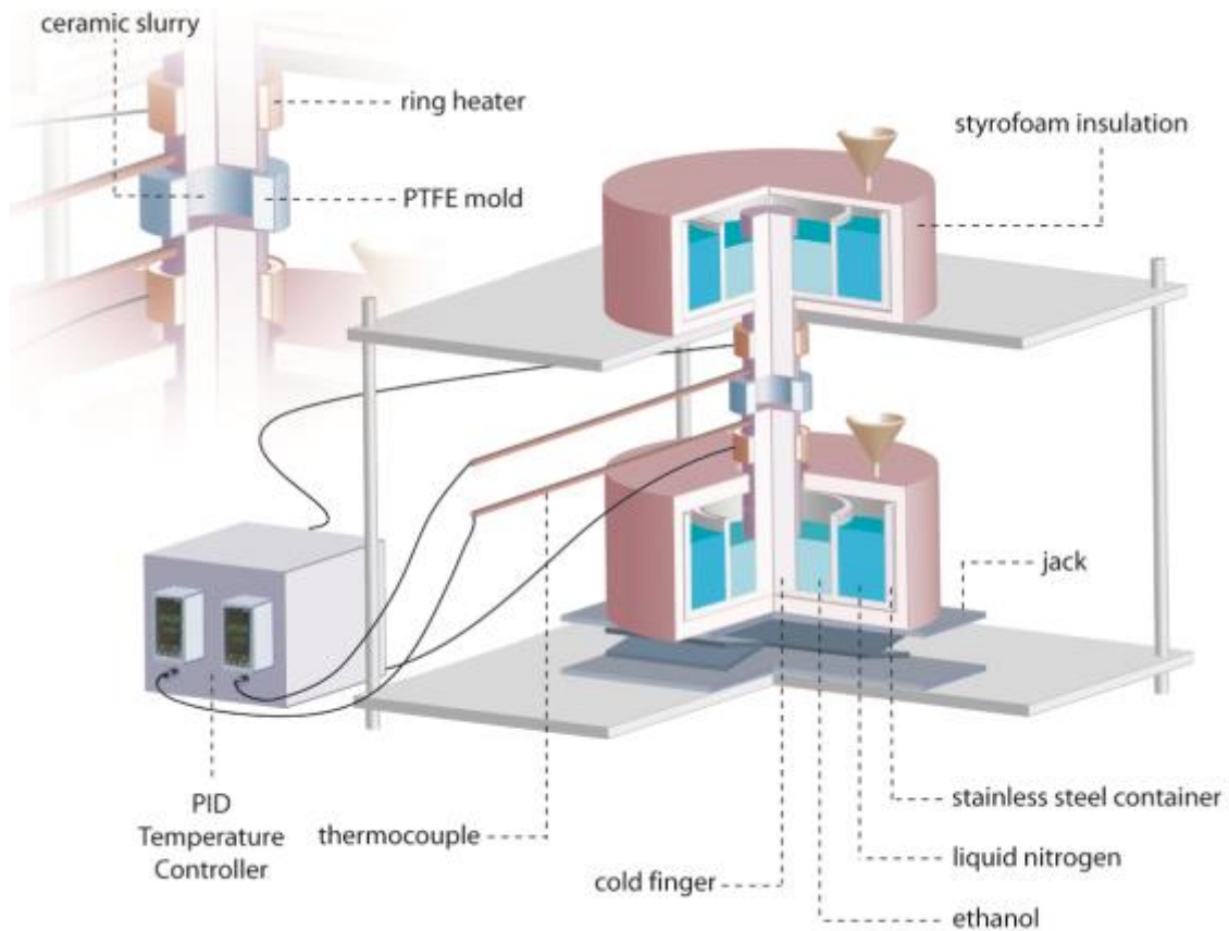
Figure 3: Schematic of the experimental apparatus employed to directionally freeze the ceramic slurries while controlling the speed of the freezing front. The ceramic slurry is poured into a Teflon mold placed between two copper cold fingers whose temperature is controlled by liquid nitrogen baths and ring heaters.
