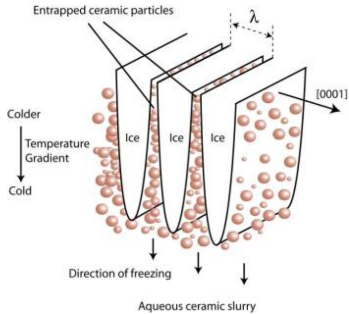
Figure 1: Pattern formation and particles segregation during freeze casting of ceramic slurries. The ice platelets grow in a direction perpendicular to the c-axes of hexagonal ice. The wavelength of the structure is defined by \lambda .
