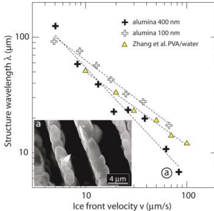
Figure 7: Variation of structure wavelength vs. ice front velocity, for samples with 64 % total porosity. The samples were frozen using only the bottom cold finger whose temperature was decreased at a constant rate (ranging between 0.1 and 10°C/min). The only exception is the sample with \sim 2 \mu\text{m} lamellae thickness where both the top and bottom cold fingers were cooled at 2 °C/min in order to maintain a constant temperature gradient of \sim 1 \text{ }^\circ\text{C/cm} . The plots can be fitted with power laws, with exponents of 1 (alumina 400nm) and 2/3 (alumina 100nm and PVA/water). Comparison of the plots is discussed in the final section. A SEM micrograph of the sample with the smallest lamellae thickness achieved in this study is shown in the insert (a), cross-section parallel to the ice front. Lamellae thickness is \sim 2 \mu\text{m} . Each value on the graph is an average of >100 measurement of wall thickness in cross section, using SEM micrographs. Error bars were not added on the graph since on a log scale, error bars were smaller than the symbols.
