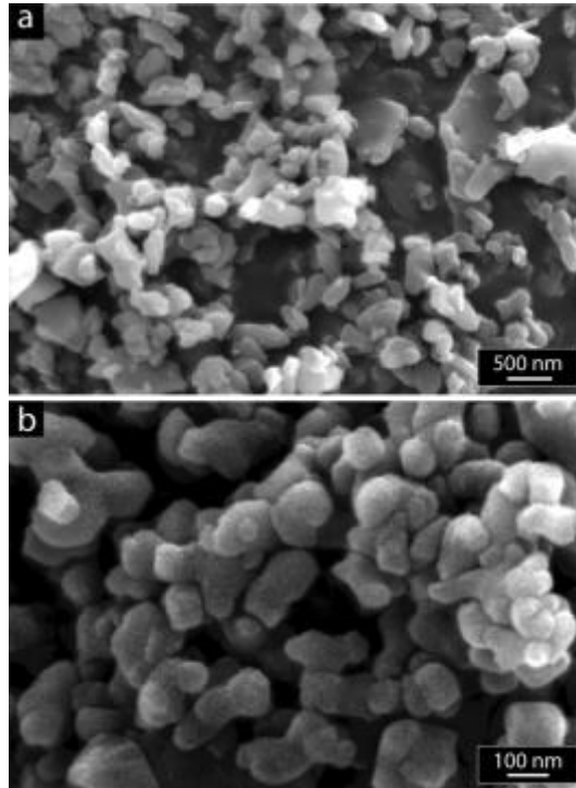
Figure 2: SEM micrographs of the ceramic powders used in this study: (a) Ceralox SPA and (b) Fine (~100 nm) alumina powder prepared according to reference [17].
