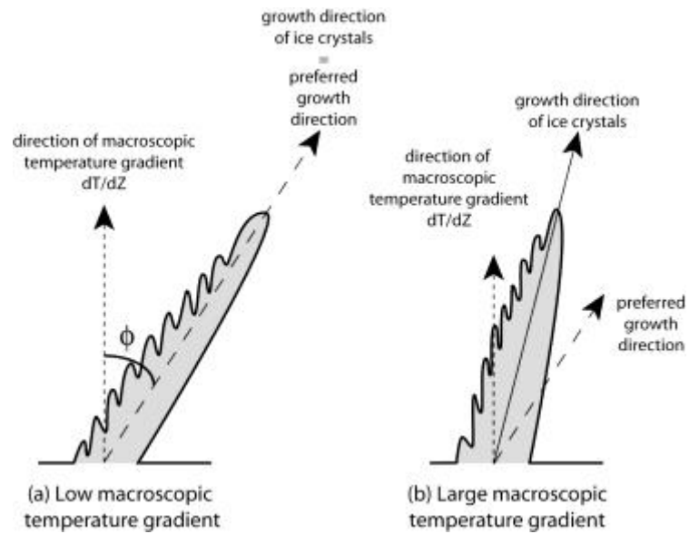
Figure 10: Growth direction of ice crystals and relationships with imposed macroscopic temperature gradient and preferred growth direction.
