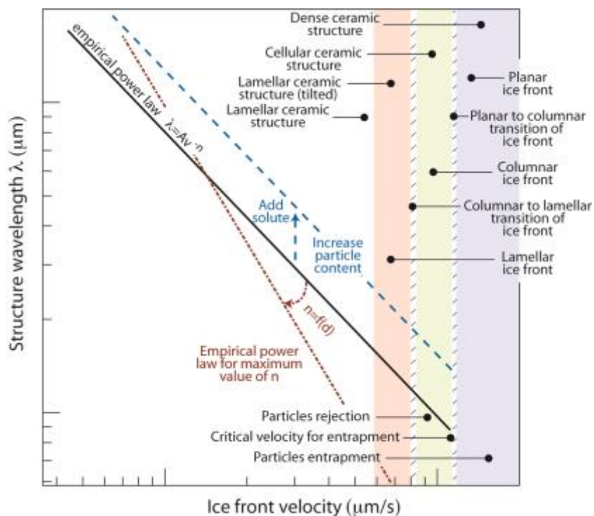
Figure 13: Strategies and limits for controlling the structure: schematic plot of wavelength vs. ice front velocity. The exponent n of the empirical law is dependent on the particle size d , though the function n = f(d) is not monotonic; an optimum of d is encountered where the exponent n is maximum. Very fast cooling rates, region (a), will result in the ice front trapping the particles and the formation of a dense material as the one observed in the bottom layer of Figure 9. When the velocity is decreased below the critical value for particle entrapment, v_c , the particles are expelled from the growing ice but if the speeds are fast enough the ice will grow with a columnar microstructure, region (b). Slower velocities will result in the formation of lamellar ice. However, if the velocity is still fast or, equivalently, the
