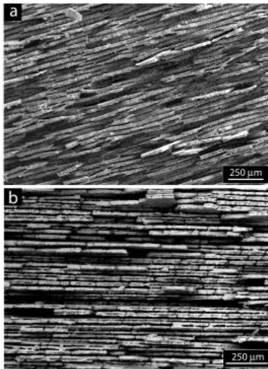
Figure 5: SEM micrographs of homogeneous lamellar alumina cross-sections. (a) Parallel to the ice front (b) Perpendicular to the ice front.
