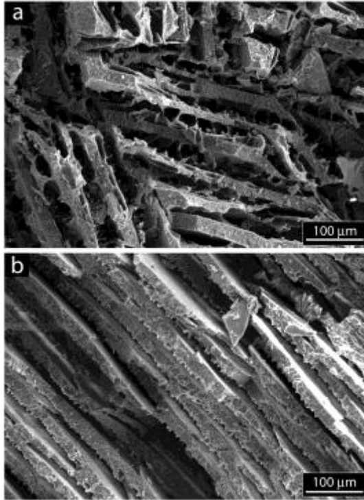
Figure 4: SEM micrographs of the porous structure: (a) Isotropic vs. (b) Anisotropic microstructure. Cross-section parallel to ice front.
