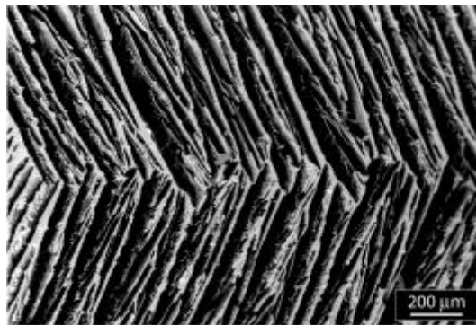
Figure 11: SEM micrograph showing tilting of the lamellae due to the effect of anisotropic interface kinetics. Cross-section perpendicular to ice front. In this case, the sample was frozen very fast using the top and bottom cold fingers to set a very small gradient, so that the crystals started on both sides almost simultaneously and joined in the middle of the sample. The tilting ( 15\text{-}20^\circ ) is clearly visible.
