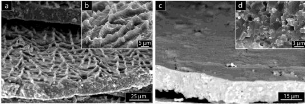
Figure 6: SEM micrographs of lamellae surface features: (a) Rough side with (b) Details in insert and (c) Smooth side. (d) Detail of the fracture surface of a lamella, the microstructure shows almost no residual porosity. The microstructure obtained after controlled solidification reveals that only one side of the lamellae is covered with dendritic-like features, the other side remaining flat. This behavior is related to the anisotropic interface kinetics.
