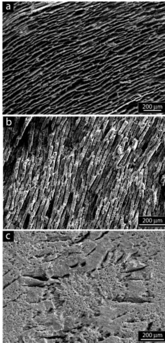
Figure 8: SEM micrograph showing the influence of water content in the slurry on the microstructure. Cross-section parallel to ice front. Total porosity of (a) 70 % (b) 40 % (c) 24 %.
