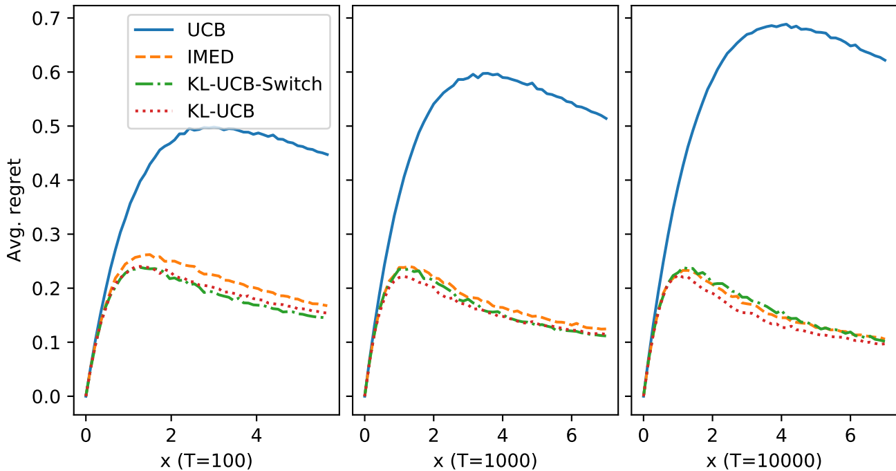
Normalized Average regret (Normalized for 5000 rounds)
