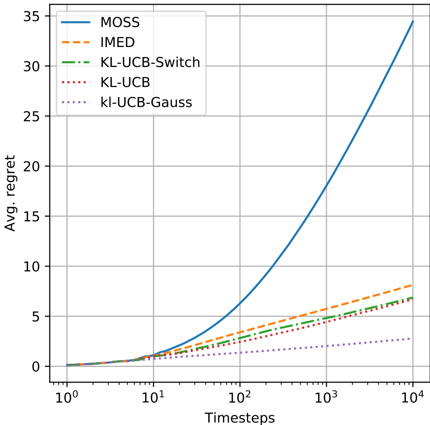
Average regret (Normalized for 10000 rounds)
