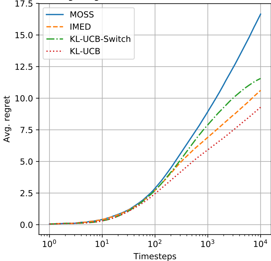
Average regret (Normalized for 10000 rounds)
