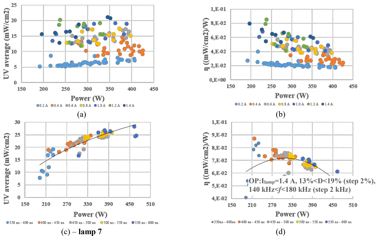
Figure 9 research of the “optimal” current pulses for the best 4 bulbs: sweep of current pulses magnitude:(a) and (b) – sweep of the current pulses duration (c) and (d)
