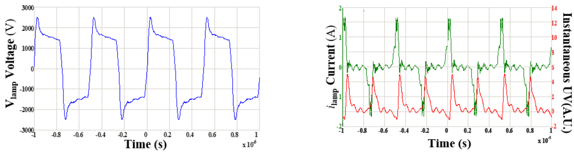
Figure 4 experimental waveforms: v_{lamp} (blue) and i_{lamp} (green), UV (red)
