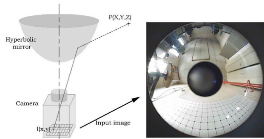
Figure 1. Omnidirectional sensor and omnidirectional image.
