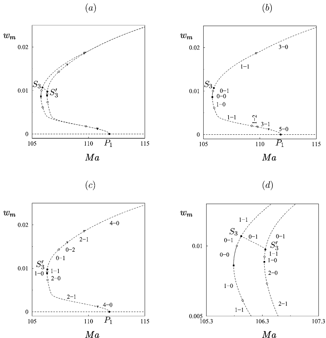
FIG. 22. (a)–(d) Closer view of Fig. 21 showing exchange of stability between the two branches emerging from P_1 . Parameters are \epsilon=1 , A=1.5 , and Pr=1 . Resolution is N_z=12 , n_x=n_y=6 , and n_z=10 .
