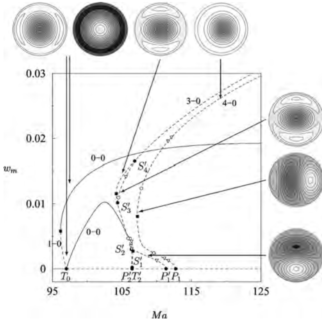
FIG. 13. Bifurcation diagram showing the maximum of the vertical velocity w_m as a function of the Marangoni number Ma . Snapshots show isovalues of the vertical velocity in the midplane of the cylinder. Parameters are \epsilon=0.98 , A=1.5 , and Pr=1 . Resolution is N_e=12 , n_x=n_y=n_z=10 .
