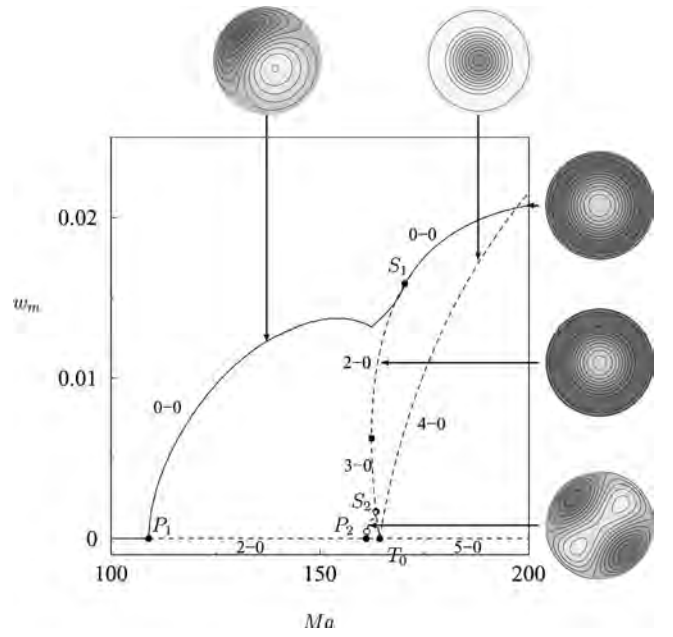
FIG. 3. Bifurcation diagram showing the maximum of the vertical velocity w_m as a function of the Marangoni number \text{Ma} . Snapshots show isovals of the vertical velocity in the midplane of the cylinder. The orientation of the m \neq 0 states is nominally arbitrary. Parameters are \epsilon=1 , A=1 , and \text{Pr}=1 . Resolution is N_e=12 , n_x=n_y=n_z=10 .
