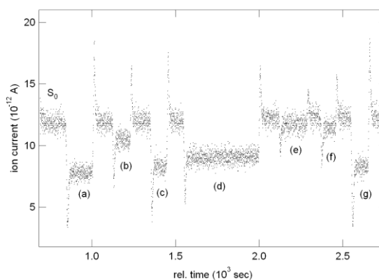
Figure 3. Typical NO 2 signal ( m/z=46 ) observed for the uptake of NO 2 gas on solid catechol in the presence of light. Experimental conditions are 0% RH, p=760 Torr and T=298 K. [\text{NO}_2]_0=1 \times 10^{15} molec. \text{cm}^3 ; injector length L (in cm) is (a) 32.5; (b) 13.8; (c) 26.0; (d) 19.8; (e) 6.5; (f) 10.5; (g) 33.8. \gamma = 2.1 \times 10^{-6}
