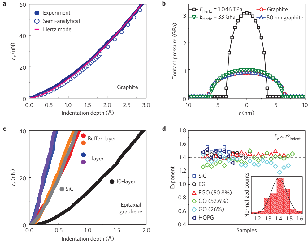
Figure 2. Experimental, SAM-simulated and Hertz indentation curves. a , Experimentally measured indentation curves in HOPG (filled circles), semi-analytical model simulations of indentation in graphite (open circles), and Hertzian fitting (continuum line) of the indentation curves on HOPG. The indenting tip radius was 100 nm. b , Contact-pressure distribution profiles for Hertz contacts and SAM simulations of indentation in graphite. Note that for bulk graphite and for a graphite film 50 nm thick, the SAM simulations and the contact distribution profiles almost overlap. c , Experimental indentation curves on 10-layer-thick EG, 1-layer-thick EG, buffer-layer EG, and SiC. d , Statistical analysis of exponent number b in the fitting function F_z = C \cdot z_{\text{indent}}^b . For EGO and GO, the RH is indicated. b_{\text{average}} is 1.40.
