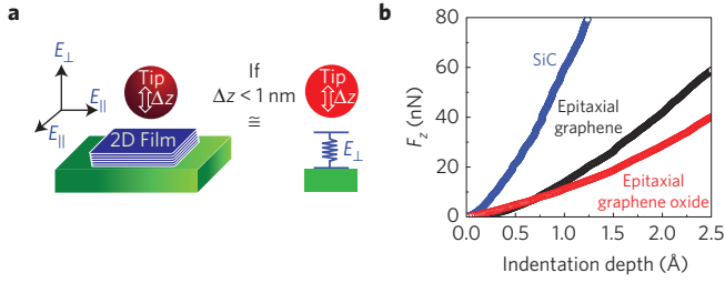
Figure 1. Modulated nanoindentation experiments. a , Schematic diagram of the experimental set-up, where a spherical AFM tip vibrates while indenting a few-layer-thick film of graphene or GO. b , Experimentally measured indentation curves for single-crystal SiC, 10-layer-thick EG, and 10-layer-thick EGO. All three curves were obtained with the same AFM tip, R=114 nm.
