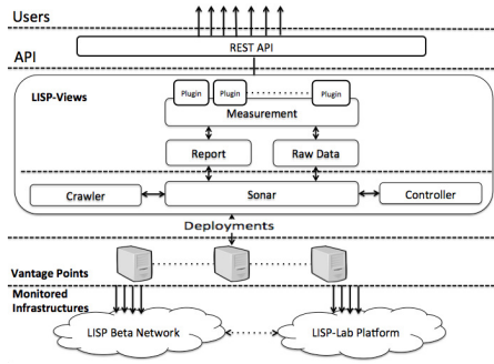
FIGURE 1: Monitoring Architecture.
