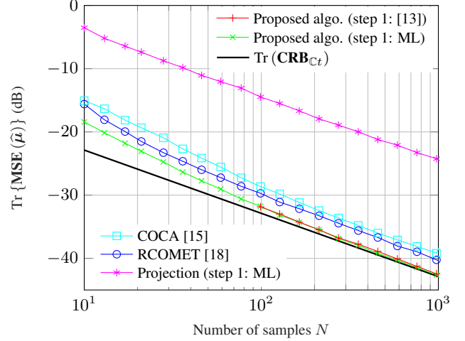
Fig. 2. Efficiency simulation
