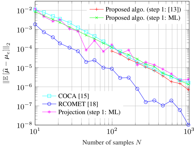
Fig. 1. Bias simulation
