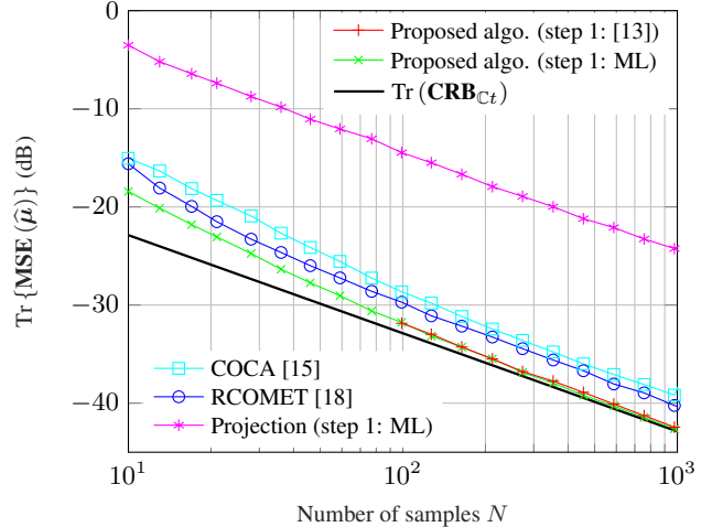
Fig. 2. Efficiency simulation
