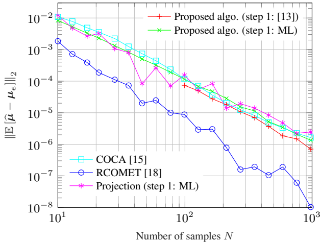
Fig. 1. Bias simulation
