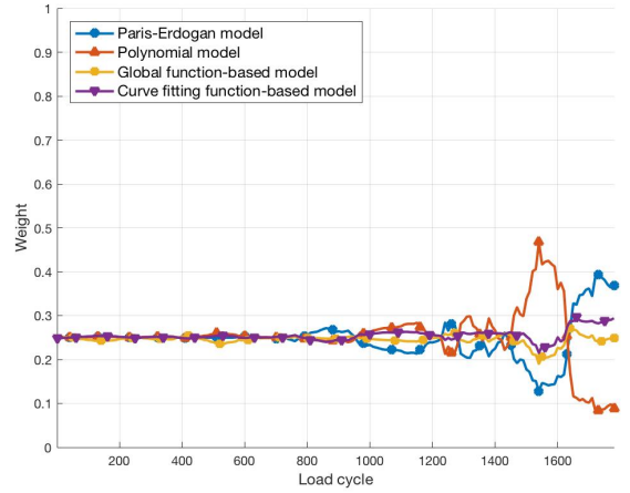
Figure 2. Dynamic ensemble weights of the individual models.
