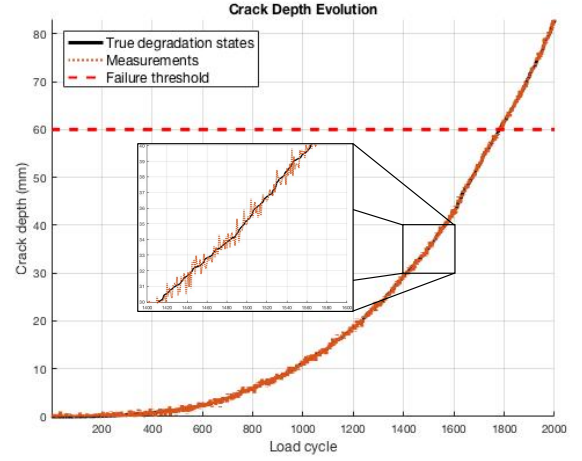
Figure 1. Simulated crack depth evolution.
