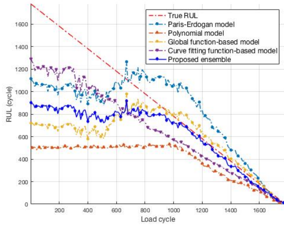
Figure 4. RUL predictions based on the individual models and the proposed ensemble.
