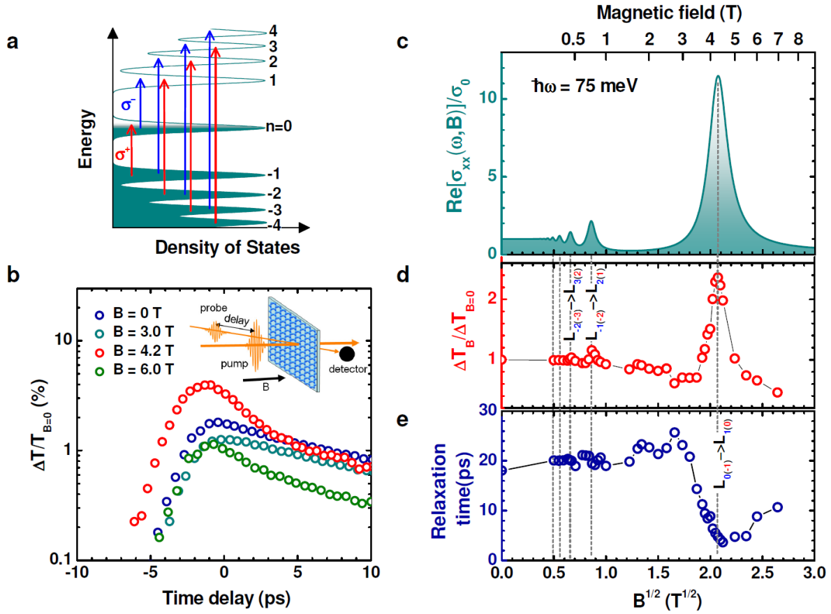
Figure 1: Pump-probe spectroscopy on graphene with linearly polarized radiation. a , Landau level spectrum of graphene with allowed dipole transitions for \sigma^- and \sigma^+ -radiation. b , Pump-probe signals for different magnetic fields. In the inset the pump-probe experiment involving linearly polarized beams is depicted. In this case, transitions allowed for \sigma^- -radiation as well as \sigma^+ -radiation are excited and probed. c , The dynamic conductivity, which is proportional to the absorption, of one graphene layer. The calculation, as well as all experimental data in the other panels, corresponds to a photon energy of 75 meV. d , B-dependent pump-induced maximum transmission change normalized to the case at zero magnetic field. e , Initial decay time of the pump-probe signal for varied magnetic fields.
