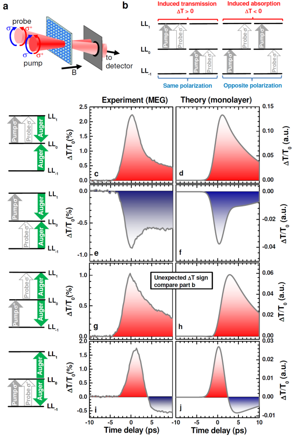
Figure 2: Pump-probe spectroscopy on graphene with circularly polarized radiation. a , Configuration of the experiments for pumping and probing with \sigma^- and \sigma^+ -radiation. b , Pumping and probing with same polarization results in induced transmission, while applying opposite polarization results in induced absorption. c , e , g , i , Experimental pump-probe signals for all four combinations of pumping and probing with \sigma^- and \sigma^+ -radiation. Blue and red shaded regions highlight positive and negative DTS, respectively. d , f , h , j , Differential transmission calculated by microscopic theory for all four combinations of pumping and probing with \sigma^- and \sigma^+ -radiation. The diagrams left of the panels indicate the polarization of pump and probe beam as well as the dominating Auger scattering process, i.e. either inward or outward Auger scattering.
